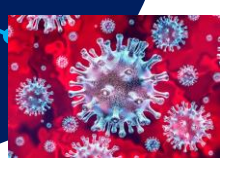
Quantitative Chemistry
