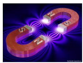
Magnetism
